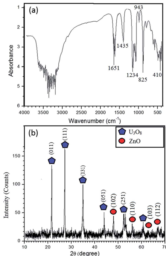
Fig. 1 (a) FT-IR spectrum of \text{UO}_2(\text{OH})_2/\text{Zn}(\text{OH})_2 . CTAB (b) XRD pattern of the synthesized \text{U}_3\text{O}_8@\text{ZnO} nanocomposite.
