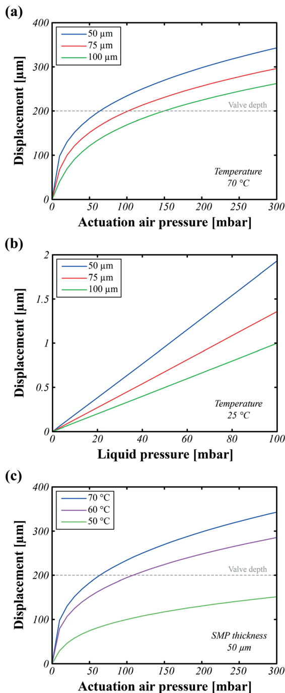
Fig. 3 Optimization of the active tri-layer thickness using FEM simulations, comparing 50 µm, 75 µm, and 100 µm thick SMP layers. (a) Displacement of the center of the membrane versus actuation air pressure in the hot state. (b) Displacement of the center of the membrane versus liquid pressure in the cold state, reporting how much the membrane moves due to liquid pressure when the air pressure is off. (c) Displacement of the center of a 50 µm thick membrane versus actuation air pressure for several temperatures, showing larger motion when the SMP is hotter, and hence softer.
