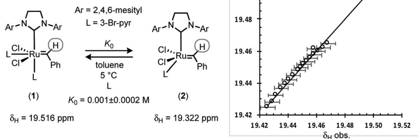
Fig. 7 ^1\text{H} NMR analysis of the chemical shift of the benzylidene-CH in G-III-Br in d_8 -toluene at 5^\circ\text{C} as a function of concentration of 1 ( [\text{Ru}]_{\text{tot}} = 2.1 to 9.7 \text{ mM} ) and 3-Br-pyridine ( 8.9 – 89 \text{ mM} at [\text{Ru}]_{\text{tot}} = 8.33 \text{ mM} ). Linear regression of the observed (x-axis) time-average population-weighted ( 1 + 2 ) chemical shift of the benzylidene-CH against that calculated (y-axis) when K_0 = 0.001 \text{ M} , \delta_1 = 19.516 \text{ ppm} and \delta_2 = 19.322 \text{ ppm} , referenced against residual d_7 -toluene \text{CHD}_2 = 2.128 \text{ ppm} . Correlation: \delta_{\text{calc.}} = 0.9981(\delta_{\text{obs.}}) + 0.0361 ; RMSE, \pm 0.00005 , yielding K_0 = 0.001 \pm 0.0002 \text{ M} . Error bars in \delta_{\text{obs.}} are at 0.005 \text{ ppm} .
