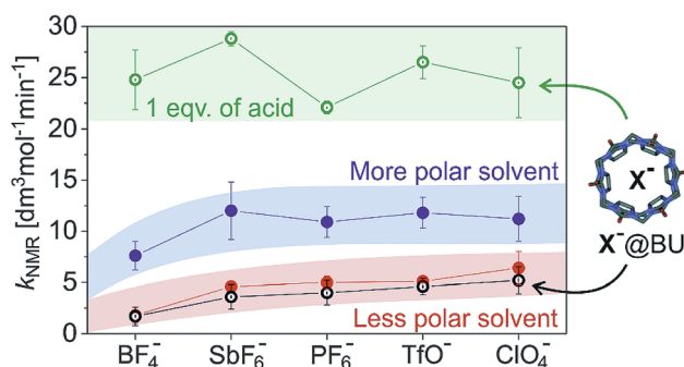
Fig. 2 Total rates ( k_{\text{NMR}} = k_1 + k_2 ) for methanol addition to 1-phenylpropyne catalysed by different (IPr)AuX salts ( X^- is indicated on the x-axis). The experiments were performed in a mixture of methanol and dichloromethane: 1 : 2.4 (red, black) and 1 : 0.08 (blue, green), respectively. The hollow points refer to the experiment with addition of 1 equivalent of Bn-BU (black) or iPr-BU*H 2 SO 4 (green) with respect to the concentration of the gold catalyst.
