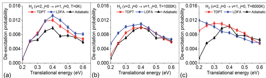
Fig. 7 Vibrational deexcitation probabilities from H_2 ( v = 2, j = 0 ) to H_2 ( v = 1, j = 0 ) simulated by MD, MDEF(LDFA), and MDEF(TDPT), with electronic temperatures of 0 K (a), 1000 K (b), and 6000 K (c).
