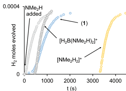
Fig. 4 Time course plot for dehydrogenation of \text{H}_3\text{B-NMe}_2\text{H} [0.072 M, 298 K, 1,2- \text{F}_2\text{C}_6\text{H}_4 solvent] using complex 1 (2 mol%), plus 1 equivalent \text{NMe}_2\text{H} , [\text{H}_2\text{B}(\text{NMe}_2\text{H})_2][\text{BAR}^{\text{F}}_4] or [\text{NMe}_2\text{H}_2][\text{BAR}^{\text{F}}_4] . \text{H}_2 as measured by \text{H}_2 eudiometer.
