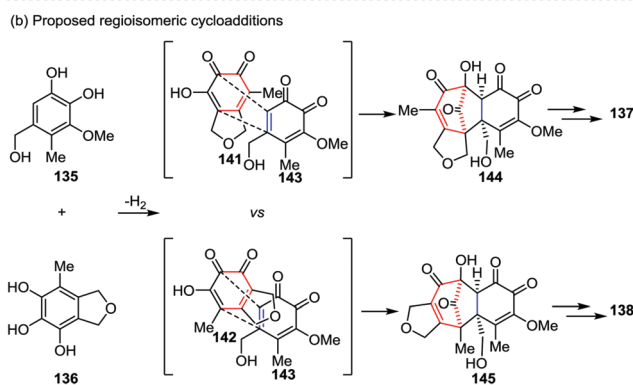
Scheme 23 (a) Total synthesis of epicolactone and isoepicolactone by Trauner and co-workers. (b) Proposed mechanism for the divergent [5+2] cycloaddition.
