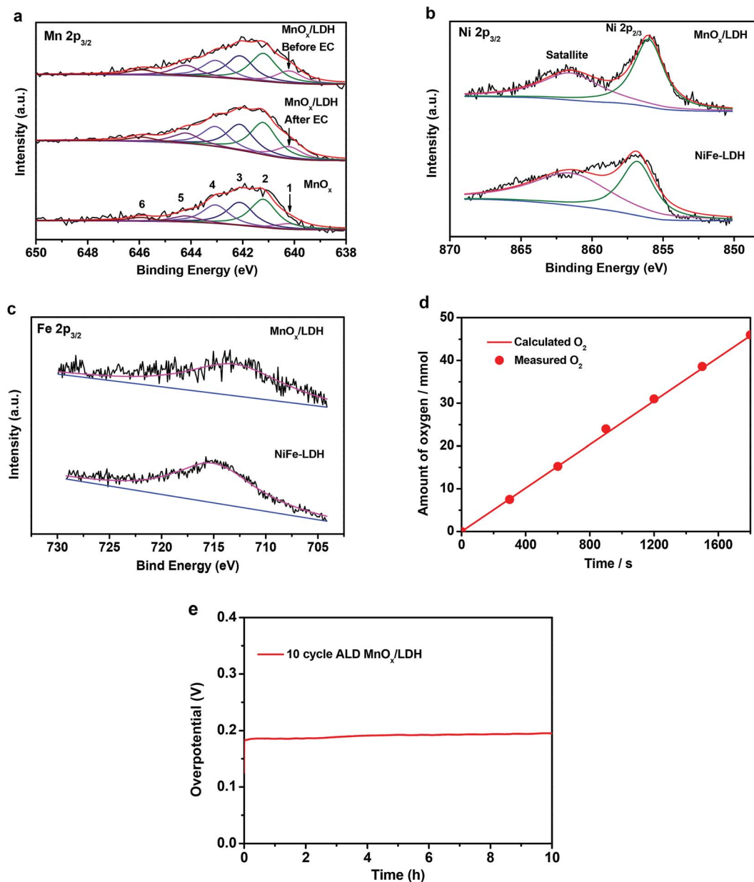
Fig. 5 XPS spectra of Mn 2p_{3/2} (a), Ni 2p_{3/2} (b) and Fe 2p_{3/2} (c) core-level photoemissions for the 10-cycle \text{MnO}_x/\text{LDH} (before and after OER testing) and original NiFe-LDH samples. Peak 1 of each spectra fitting is labelled with a black arrow in (a). (d) Generated \text{O}_2 gas molar quantities as a function of time overlaid with the calculated quantities of evolved \text{O}_2 assuming 100% faradaic efficiency. (e) Chronopotentiometric measurements recorded for 10-cycle \text{MnO}_x/\text{LDH} electrocatalysts at a constant current density of 10 \text{ mA cm}^{-2} .
