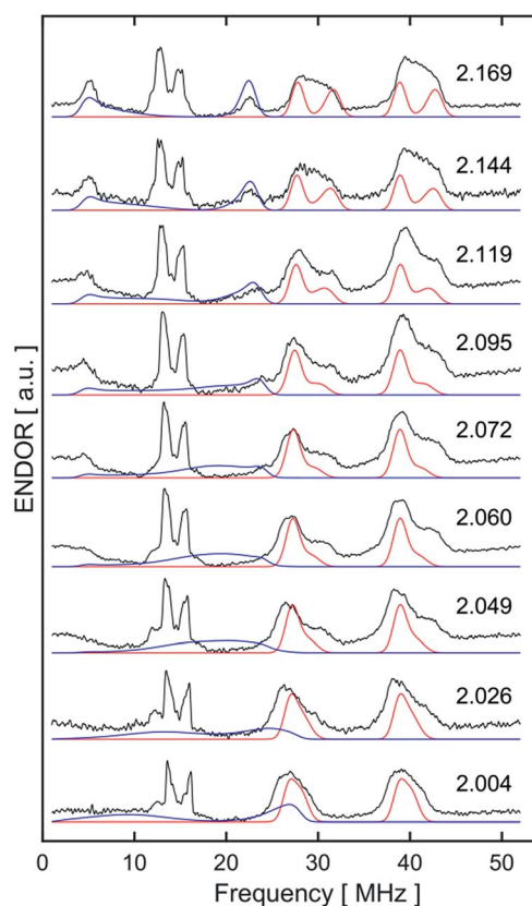
Fig. 6 X-band Davies ENDOR spectra of [\mathbf{1} \cdot \text{H}_2]^+[\text{BAR}_4^F]^- at 2.5 mM in 7 : 1 PhMe : DFB, collected at nine field positions as indicated by g -value along the right side. The sample was a frozen glass at 20 K and measured with pulse lengths of \pi/2 = 40 ns and \pi_{\text{inv}} = \pi = 80 ns, \pi = 300 ns, RF pulse = 16 \mu\text{s} , and 1 \mu\text{s} before and 2 \mu\text{s} after the RF pulse, with stochastic frequency stepping. The microwave frequency was 9.7621 GHz. Experimental data is in black, while simulations of ^{31}\text{P} values are red, and simulations of ^1\text{H} are in blue (as discussed in main text).
