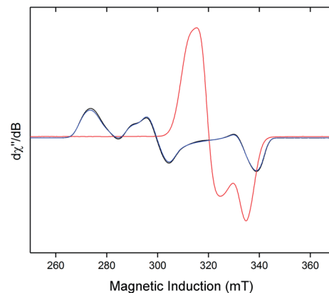
Fig. 7 Reversible binding of H 2 by [\mathbf{1}]^+[\text{BAR}_4^F]^- in the solid-state: CW X-band ESR spectra of powdered [\mathbf{1}]^+[\text{BAR}_4^F]^- under Ar (black), followed by evacuation and subsequent admission of H 2 (1 bar, [\mathbf{1} \cdot \text{H}_2]^+[\text{BAR}_4^F]^- , pink), and sequential evacuation to 10 −3 mbar and backfill with Ar (blue). All spectra recorded at 40 K.
