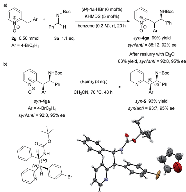
Scheme 3 Larger scale reaction with lower catalyst loading and removal of N-oxide moiety. Single-crystal X-ray analysis of 5 . Thermal ellipsoids are shown at 50% probability.
