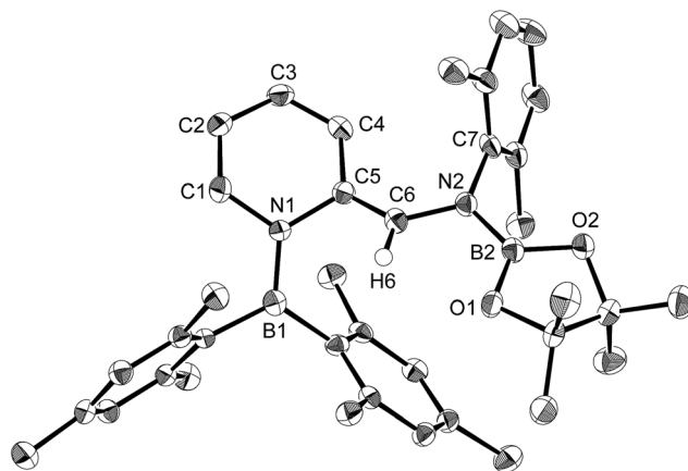
Fig. 4 Molecular structure of 5 (thermal ellipsoids set at 50% probability; hydrogen atoms except for H6 omitted for clarity). Selected bond distances (Å), angles ( ^\circ ) and dihedral angles ( ^\circ ): B1–N1 1.428(4), N1–C1 1.425(4), C1–C2 1.334(5), C2–C3 1.449(5), C3–C4 1.344(5), C4–C5 1.467(5), N1–C5 1.457(4), C5–C6 1.354(4), C6–N2 1.412(4), N2–B2 1.425(5), B2–O1 1.376(4), B2–O2 1.386(4); B1–N1–C5 124.2(3), N1–C5–C6 114.8(3), C5–C6–N2 130.0(3), C6–N2–B2 118.6(3); B1–N1–C5–C6 -45.5(4) , N1–C5–C6–N2 169.6(3) , C5–C6–N2–B2 -167.2(3) , C6–N2–B2–O1 -11.3(5) .
