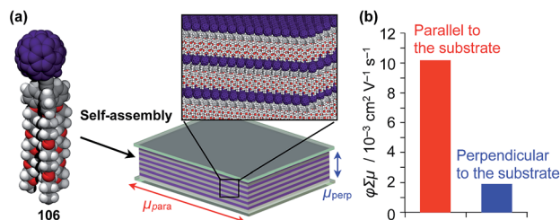
Fig. 17 (a) Schematic structure of an oriented 2D assembly of C 60 units achieved by a tripodal triptycene-based 2D supramolecular scaffold ( 106 ) and (b) its maximum transient conductivities ( \sigma\Sigma\mu ) sandwiched between quartz substrates along directions parallel (red) and perpendicular (blue) to the substrate as determined by flash-photolysis time-resolved microwave conductivity measurements.
