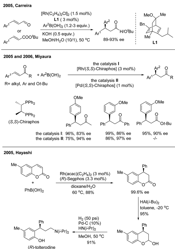
Scheme 3 The enantioselective 1,4-addition of arylboronic acids to \beta -aryl substituted unsaturated carbonyl derivatives.
