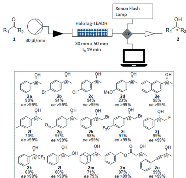
Fig. 4 Asymmetric reduction of ketones by using the immobilized HaloTag- Lb ADH in flow. Reaction conditions: ketones 1a–1o (50 mM), NADPH (0.5 mM), 2-propanol (10 vol%), THF (30 vol%), KPi 50 mM (pH 7.0), MgCl 2 ·H 2 O (1 mM), flow rate (30 μl min -1 ). Isolated yields after purification. The ee were determined by GC or HPLC as described in the experimental procedure.
