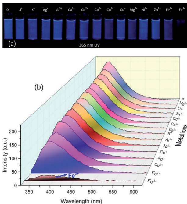
Fig. 4 (a) Photographs taken under 365 nm UV light and (b) fluorescence spectra of PASAS aqueous solution (5 mg mL -1 ) in the presence of various metal ions (2 × 10 -3 mol L -1 ).
