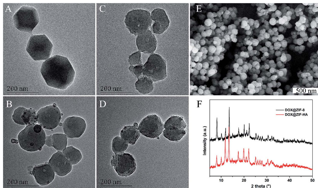
Fig. 2 TEM images of (A) pure ZIF-8, (B) DOX@ZIF-8, (C) DOX@ZIF-PDA and (D) DOX@ZIF-HA nanoparticles. (E) An FESEM image of the prepared DOX@ZIF-HA. (F) The XRD results of the prepared nanoparticles.
