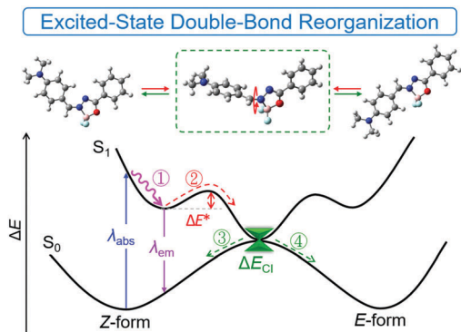
Fig. 7 A proposed model for the excited-state behavior of E/Z photoisomerization of DMA-POABP. \Delta E^* denotes the energy barrier from Z to E -form, and \Delta E_{Cl} denotes the energy gap of the de-excitation pathway through the conical intersection between the S_0 and S_1 states. Route ① and ② were the reorganization process in the excited state, and route ③ and ④ and \lambda_{em} were the de-excited process to the S_0 state.
