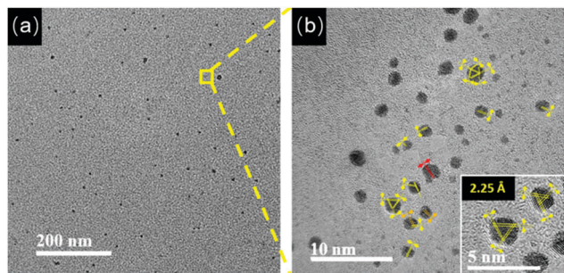
Fig. 5 (a) TEM image of the Au NCs at pH 11.0. (b) HRTEM image of the zone marked by the yellow frame in (a). (inset) Enlarged HRTEM image of the Au NCs in (b).
