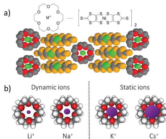
Fig. 8 Dynamic ( \text{M}^+ = \text{Li}^+ and \text{Na}^+ ) and static ( \text{M}^+ = \text{K}^+ and \text{Cs}^+ ) ionic channels in conducting \text{M}^+_{\text{x}}([\text{18}]\text{crown-6})[\text{Ni}(\text{dmit})_2]_2 salts. (a) Molecular structures and packing structure. The motional freedom of the cations affected the potential for the conduction electrons on the \pi -stack of partially oxidized [\text{Ni}(\text{dmit})_2] . (b) Dynamic and static ion environments were observed according to the size of the alkali metal ions ( \text{Li}^+ , \text{Na}^+ , \text{K}^+ , and \text{Cs}^+ ) and cavity size of the [18]crown-6 ether.
