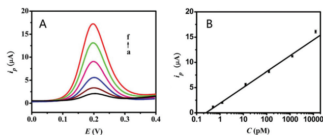
Fig. 4 (A) DPV response to 0.5, 1.25, 12.5, 125, 1250, and 12500 pM target miRNA (from a to f). (B) Plot of DPV peak current vs. logarithm of target miRNA concentration. The error bars represent the standard deviations in three different measurements for each concentration.
