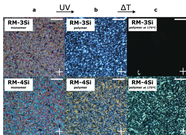
Fig. 2 POM images obtained between crossed polarizers of the LCs in a cell (a) before photopolymerization, (b) after photopolymerization, and (c) after heating the samples. Crossed polarizer axes are indicated with a cross. All scale bars: 100 μm.
