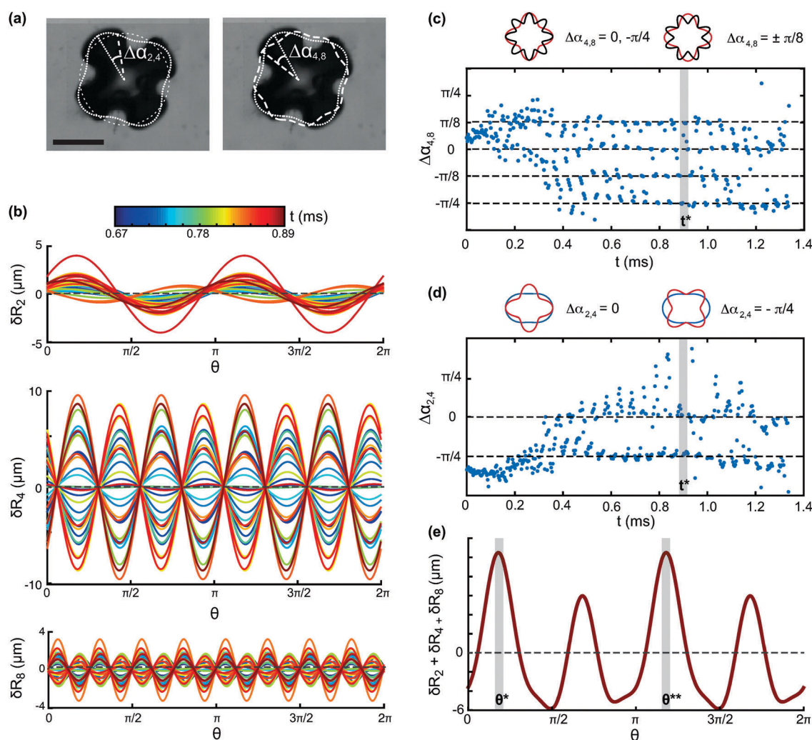
Fig. 4 (a) Contours of modes n = 2, 4 and 8 overlaid on the overall bubble shape. \Delta_{2,4} and \Delta_{4,8} are the phase differences between the modes. Scale bar: 80 \mu\text{m} . (b) Time evolution of the three modes. Different times correspond to different colour (see colorbar). (c) Time evolution of the phase difference between modes 4 and 8 , \Delta_{4,8} . The two modes align with their antinodes in phase. The shaded area corresponds to the time of desorption. (d) Time evolution of the phase difference between modes 2 and 4 , \Delta_{2,4} . The phase difference behaves erratically in time, but the two modes are aligned at the time of desorption (shaded area). (e) Superposition of modes n = 2, 4 and 8 at the time of desorption. The shaded areas mark the locations of the two desorption plumes, which are found to correspond to the locations of maximum deviation from spherical shape.
