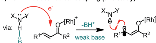
Fig. 1 Formation of C–N bonds by \beta -amination of readily available \alpha,\beta -unsaturated carbonyl compounds. Scope limitations for the PCET-induced radical coupling reported in this study: X = aryl, Y = CO 2 R, R 1 = aryl, R 2 = 2-imidazolyl.
