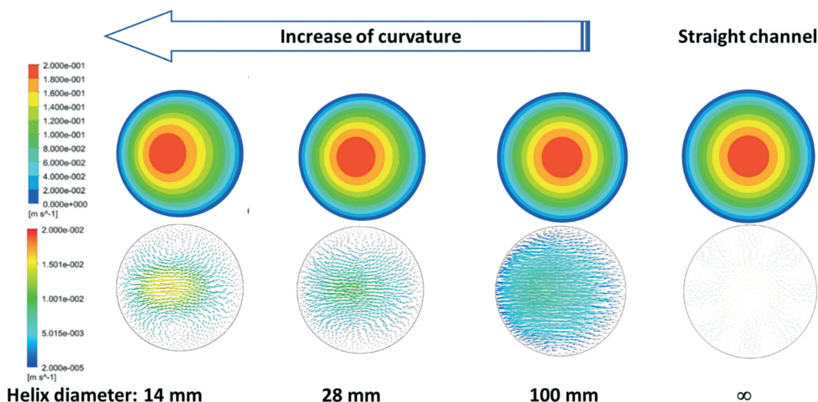
Fig. 10 Fluid dynamic simulation results of the effect of helix diameter on the formation of secondary transverse flows with an inlet velocity of 0.1 m s -1 . The upper row shows the cross section velocity magnitude contour and the bottom row shows the corresponding cross section velocity vectors.
