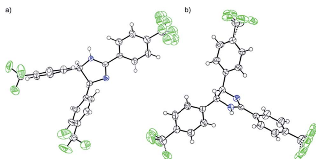
Fig. 5 ORTEP representation of the molecular structure of cis -1 (a) and trans -9 (b) at 50% probability as determined by single-crystal X-ray diffraction, which revealed that some of the -\text{CF}_3 groups can have more than one arrangement in the crystal.
