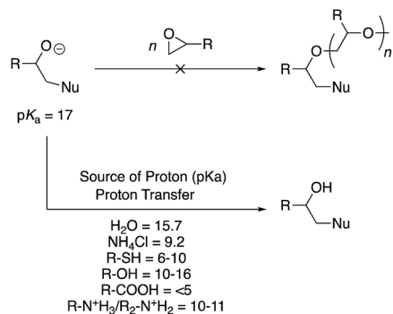
Scheme 5 The alkoxide anion is a strong base and is quenched by weak acidic protons present in the system. Therefore, it cannot act as an initiator for ring-opening polymerisation of the pendent epoxide groups. The bottom shows pK_a of various functional groups, solvents, or additives that are typically present in the PGMA functionalisation reactions. Nu stands for nucleophile.
