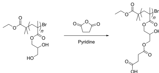
Scheme 16 Second functionalisation of hydrolyzed PGMA through ring-opening reaction with succinic anhydride by Gao and co-workers.
