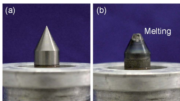
Fig. 9 (a) Photograph of a tungsten pencil-type electrode of an in-liquid plasma generator of the microwave type in an unused state; (b) photograph of a tungsten pencil-type electrode after several minutes of generating in-liquid plasma with continuous microwaves. Taken from ref. 17. Copyright 2017 by S. Horikoshi.
