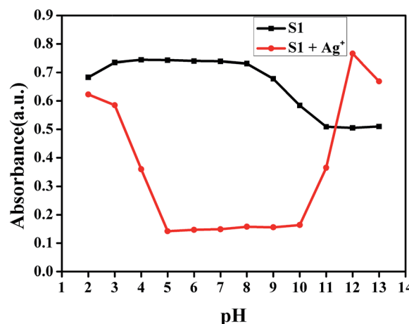
Fig. 5 pH response of S1 and S1 -Ag + in the DMSO/H 2 O (v:v = 1 : 1; buffered with HEPES) solution.
