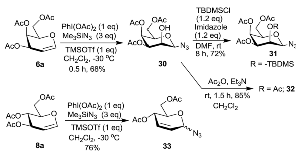
Scheme 8 Reaction of glycal derivatives 6a and 8a with PIDA- \text{Me}_3\text{SiN}_3 .
