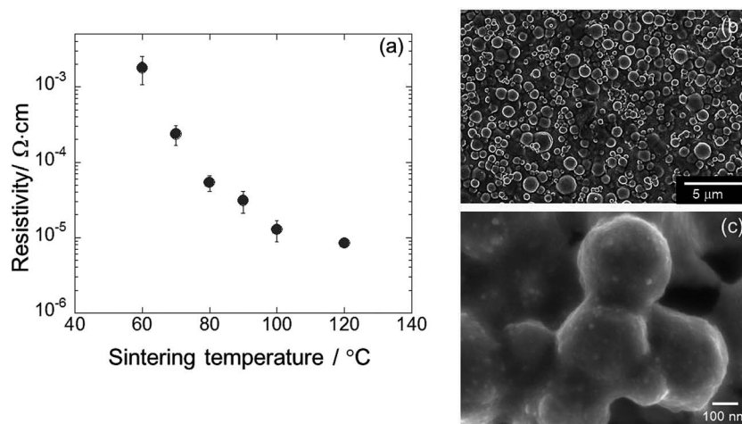
Fig. 29 (a) Change in electrical resistivity of Cu films as a function of sintering temperature. (b, c) SEM images of the sintered Cu films prepared after sintering at 80 °C. [Reprinted with permission from ref. 269 Copyright © American Chemical Society.]
