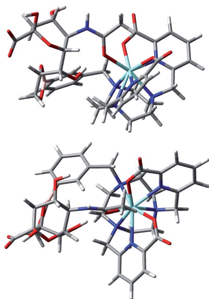
Fig. 14 Views of the hypothetical binding of the glycerol diol group to boron and cooperative ligand binding of the amide carbonyl oxygen to the metal ion in an optimised model geometry for the complex [\text{Eu} \cdot \text{L}^3 \cdot \text{sialic acid}] . 11,12
