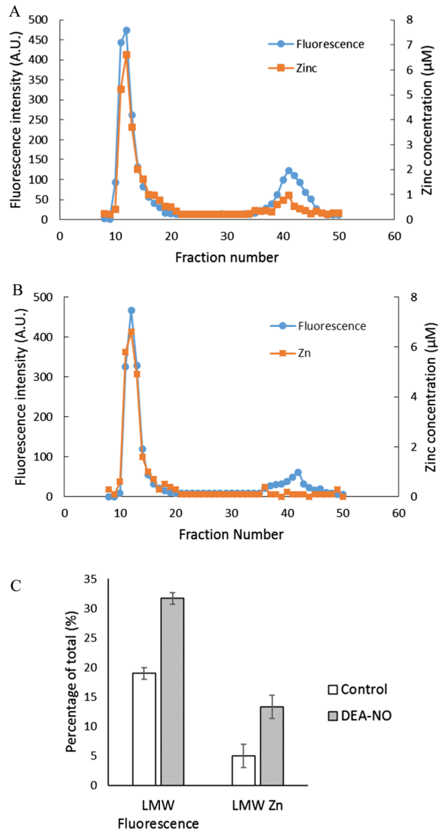
Fig. 3 Sephadex G-75 gel filtration of LLC-PK 1 cell supernatant incubated with 20 \mu M ZQee followed by 500 \mu M DEA-NO. (A) 10 8 LLC-PK 1 cells were reacted with 500 \mu M DEA-NO for 40 min following 20 \mu M ZQee for 30 min. The cells were lysed, centrifuged, and the supernatant separated using Sephadex G-75 column chromatography. The fractions were analyzed for both fluorescence and zinc. (B) Control: a parallel reaction was run under identical conditions without DEA-NO. (C) Comparison of the low molecular weight (LMW) fluorescence and zinc content between control and DEA-NO exposed cells. Error bars represent standard errors for at least three measurements.
