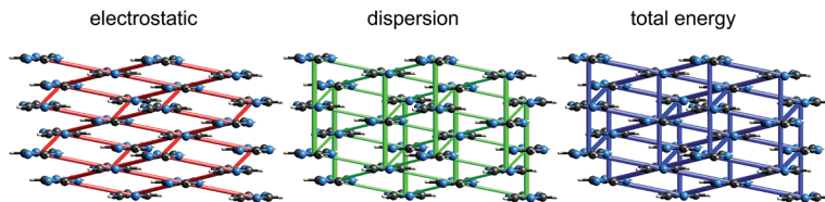
Fig. 11 s-Triazine (TRIZIN): energy frameworks for separate electrostatic (red) and dispersion (green) contributions to the total nearest neighbour pairwise interaction energies (blue). See Fig. 10 for details.
