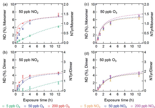
Fig. 3 NDs of protein monomer and dimer (primary y-axis), and NTyr number per monomer and dimer (secondary y-axis) plotted against reaction time in the aqueous phase reaction of BSA with O_3/NO_2 : (a) and (b) at a fixed NO_2 concentration of 50 ppb with varied O_3 concentrations, and (c) and (d) at a fixed O_3 concentration of 50 ppb with varied NO_2 concentrations. The data points and error bars represent the arithmetic mean values and standard deviations of duplicate experiments. The dashed lines are the results of the kinetic model.
