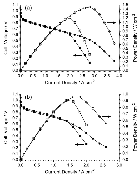
Fig. 12 The \text{H}_2/\text{O}_2 AEMFC performances of the LDPE-AEM (100 kGy) ( \bullet , \circ ) and ETFE (30 kGy) ( \blacksquare , \square ) at (a) 80^\circ\text{C} and (b) 60^\circ\text{C} : PtRu/C (50% wt Pt and 25% wt Ru) anodes and Pt/C (40% wt) cathodes (all 0.4 \text{ mg}_{\text{Pt}} \text{ cm}^{-2} loadings). The 1.0 SLPM gas supplies contained 10 ppm \text{CO}_2 contamination and were not pressurised: relative humidity (RH) = 68% for the 60^\circ\text{C} tests and RH = 100% for the 80^\circ\text{C} tests (these humidity levels were optimised for maximum performance at each cell temperature).
