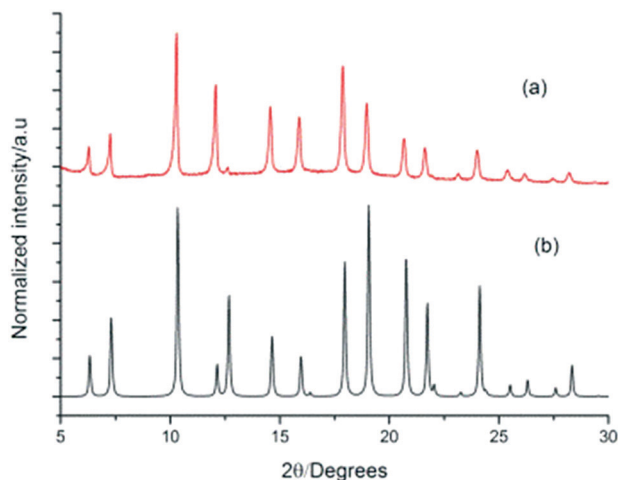
Fig. 8 PXRD of ternary co-crystal, (CC3-S 0.5 CC4-S 0.5 )-(CC13-S 0.5 CC3-S 0.25 CC4-S 0.25 ). (a) Experimental PXRD pattern, and (b) simulated PXRD pattern from single crystal structure. A close match between the patterns is observed.
