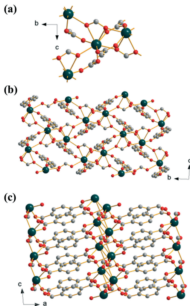
Fig. 3 Structure of (3): (a) local view of the connection of four Yb centres, (b) view along a , and (c) view along b . Atomic labelling scheme as for Fig. 1 with hydrogen atoms omitted for clarity.
