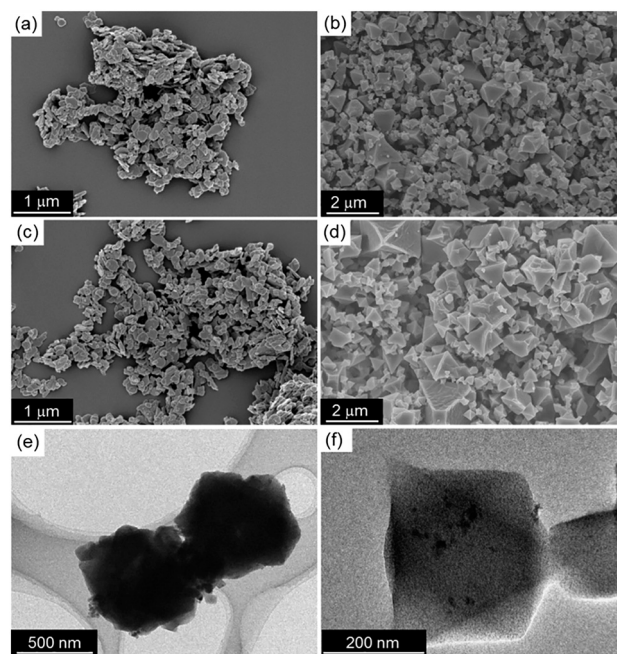
Fig. 2 SEM images of (a) \text{Fe}_3\text{O}_4@Cu_2(\text{OH})_3\text{NO}_3 , (b) \text{Fe}_3\text{O}_4@HKUST-1 , (c) \text{Cu}_2(\text{OH})_3\text{NO}_3 and (d) HKUST-1. (e and f) TEM images of \text{Fe}_3\text{O}_4@HKUST-1 .
