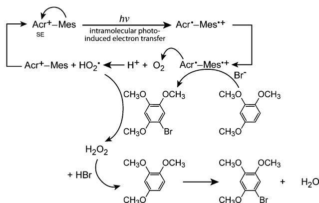
Fig. 12 Schematic representation of the photocatalytic bromination of 1,2,4-trimethoxybenzene (TMB) with 9-mesityl-10-methylacridinium ( \text{Acr}^+ - \text{Mes} ) as a catalyst. SE: Singlet excited state.
