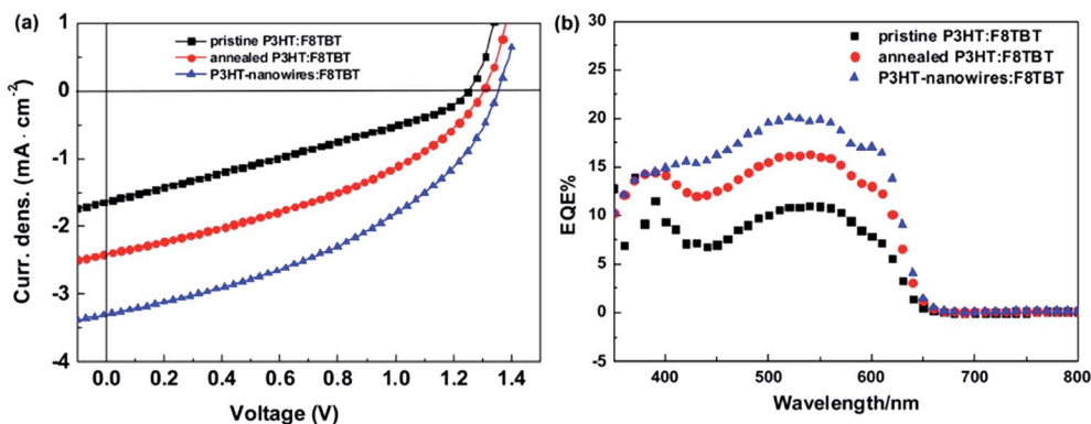
Fig. 21 (a) J - V characteristics and (b) EQE spectra of the as-cast P3HT/F88TBT (black squares), annealed P3HT/F88TBT (red circles), and P3HT-nanowire/F88TBT (blue triangles) blend solar cells under simulated AM1.5G solar light illumination with an intensity of 100 \text{ mW cm}^{-2} . Both the annealed P3HT/F88TBT and P3HT-nanowire/F88TBT blends were annealed at 140 \text{ }^\circ\text{C} for 15 min before electrode deposition. Reproduced with permission from (ref. 53). Copyright 2014, American Chemical Society.
