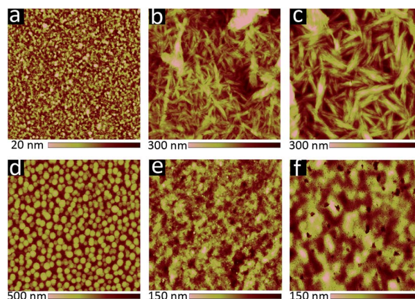
Fig. 4 10 \times 10 \mu\text{m} AFM images of active layer blends cast from 20 \text{ mg mL}^{-1} solutions; (a–c) 6:PC 71 BM active layers with (a) 0%, (b) 1%, (c) 3% DIO (v/v); (d–f) 8:PC 71 BM active layers with (d) 0%, (e) 1%, (f) 3% DIO (v/v).
