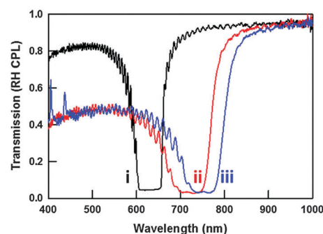
Fig. 7 Photosensitivity of t-PSCLC prepared with the photoinitiator I-907 (1 wt%). Transmission spectra at (i) 0 V (—), (ii) during application of 40 V DC (—), and during application of 40 V DC in the presence of 50 mW cm -2 of UV light (—).
