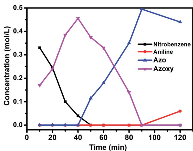
Fig. 5 Substrate and product concentration profiles as a function of the reaction time. Reaction conditions: Co–N–C catalyst: 0.7\text{ mol\%} ; \text{NaOH} ( 0.2\text{ equiv.} ); solvent: t -BuOH ( 2\text{ mL} ); 80\text{ }^\circ\text{C} ; 3\text{ MPa } H_2 .
