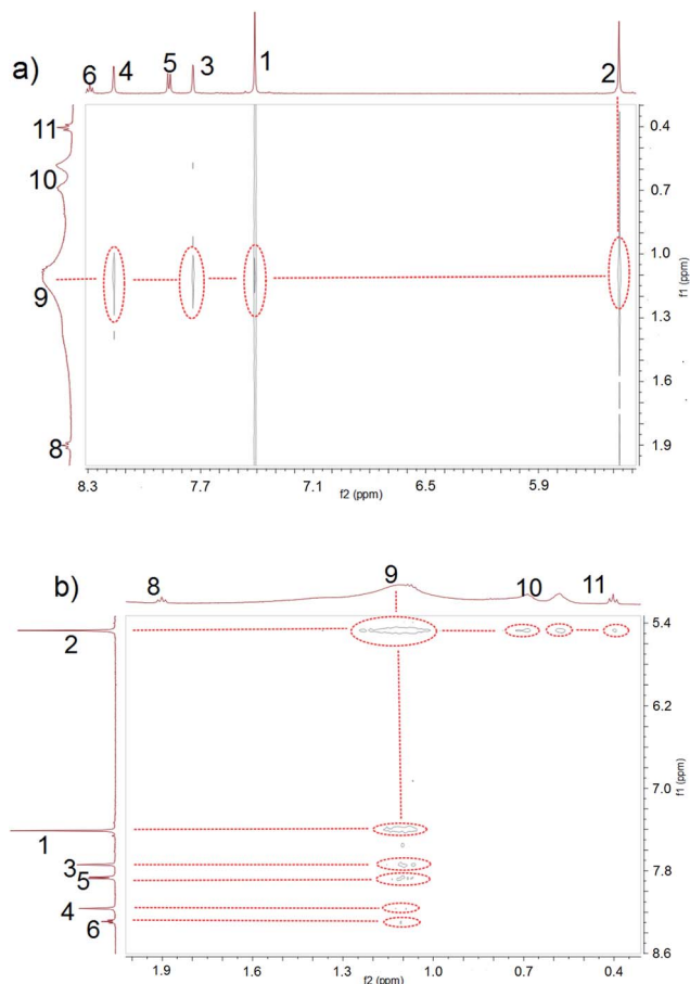
Fig. 2 Expanded views of the NOESY NMR spectra (600 MHz, D 2 O, 298 K) of 1 and 2 (each at 3.00 mM).
