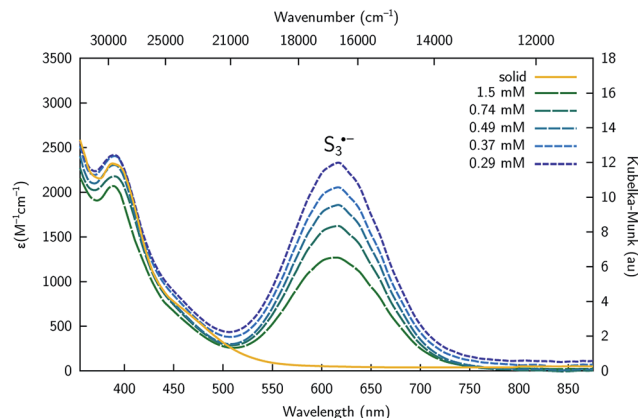
Fig. 6 UV-Vis spectra of [K_2(DMF)_3][4] in the solid state (yellow), and in DMF at 20 °C collected at varying concentration showing the presence of S_3^{2-} ( \lambda_{max} = 617 nm) in solution.
