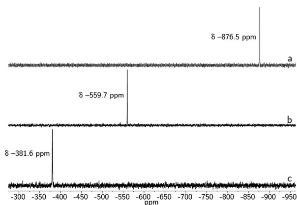
Fig. 5 ^{119}\text{Sn}\{^1\text{H}\} NMR spectra of 3 (a), 4 (b), and 1 (c) taken in DMSO- d_6 at 20 °C (149 MHz).
