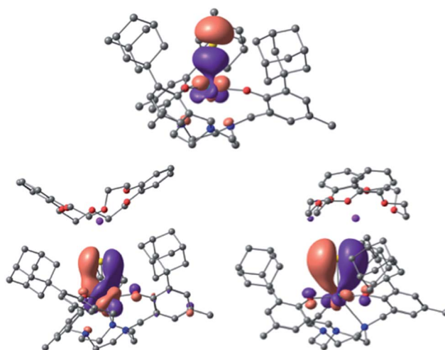
Fig. 7 U–S bonding orbitals in [[((^{\text{Ad,Me}}\text{ArO})_3\text{tacn})\text{U}\equiv\text{S}\cdots\text{K}(\text{db-18-c-6})] (3), with the \sigma (top) and the set of two \pi orbitals (bottom).
