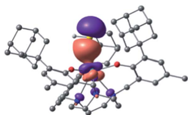
Fig. 6 Bonding \sigma orbital of [[((^{\text{Ad,Me}}\text{ArO})_3\text{tacn})\text{U-SH}] (2).
