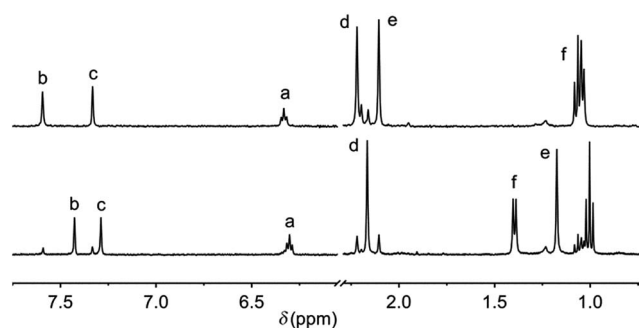
Fig. 1 Aliphatic and aromatic region in the ^1\text{H} NMR spectrum of 1a (1 mM in \text{DMSO}-d_6 ) before (top) and after (bottom) 312 nm irradiation at 20 °C for 1 h. The top spectrum was recovered upon subsequent 365 nm irradiation for 1.5 h (see Fig. S6 in the ESI†). For the proton assignment, see Scheme 1.
