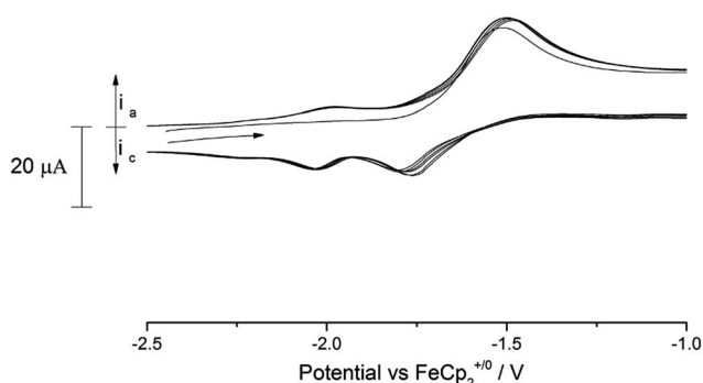
Fig. 10 Overlaid scan (4 cycles) of (9) in 0.05 M [\text{N}(\text{7Bu})_4][\text{B}(\text{C}_6\text{F}_5)_4]/ THF. Scan rate 100 \text{mV s}^{-1} .
