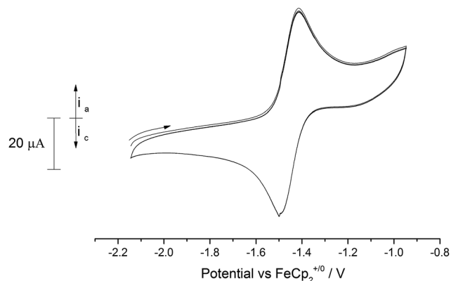
Fig. 11 Overlaid CV scans (2 cycles) of (10') in 0.1 M [\text{N}(\text{7Bu})_4][\text{PF}_6]/ acetonitrile. Scan rate 150 \text{mV s}^{-1} .
