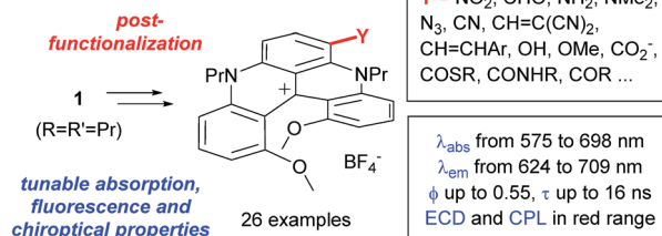
Fig. 1 Cationic aza helical chromophores and the scope of this work.
