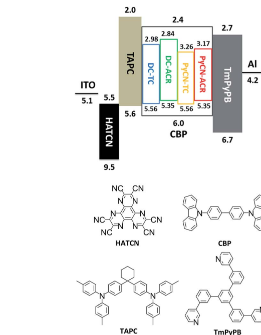
Fig. 8 Energy level diagram and molecular structures of the materials for fabricating OLED devices. The HOMO and LUMO levels of the investigated molecules were estimated by cyclic voltammetry.
